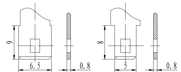
Positive terminal
